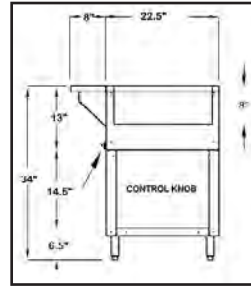
Sectional View of Hot Food Table
