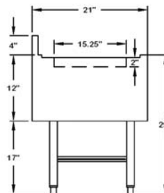
Sectional View
