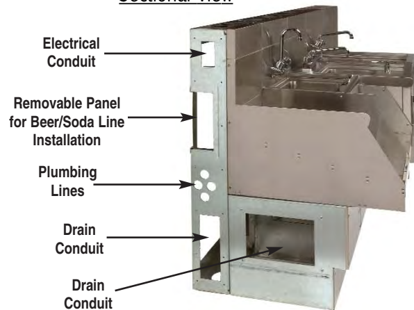
Sectional View
